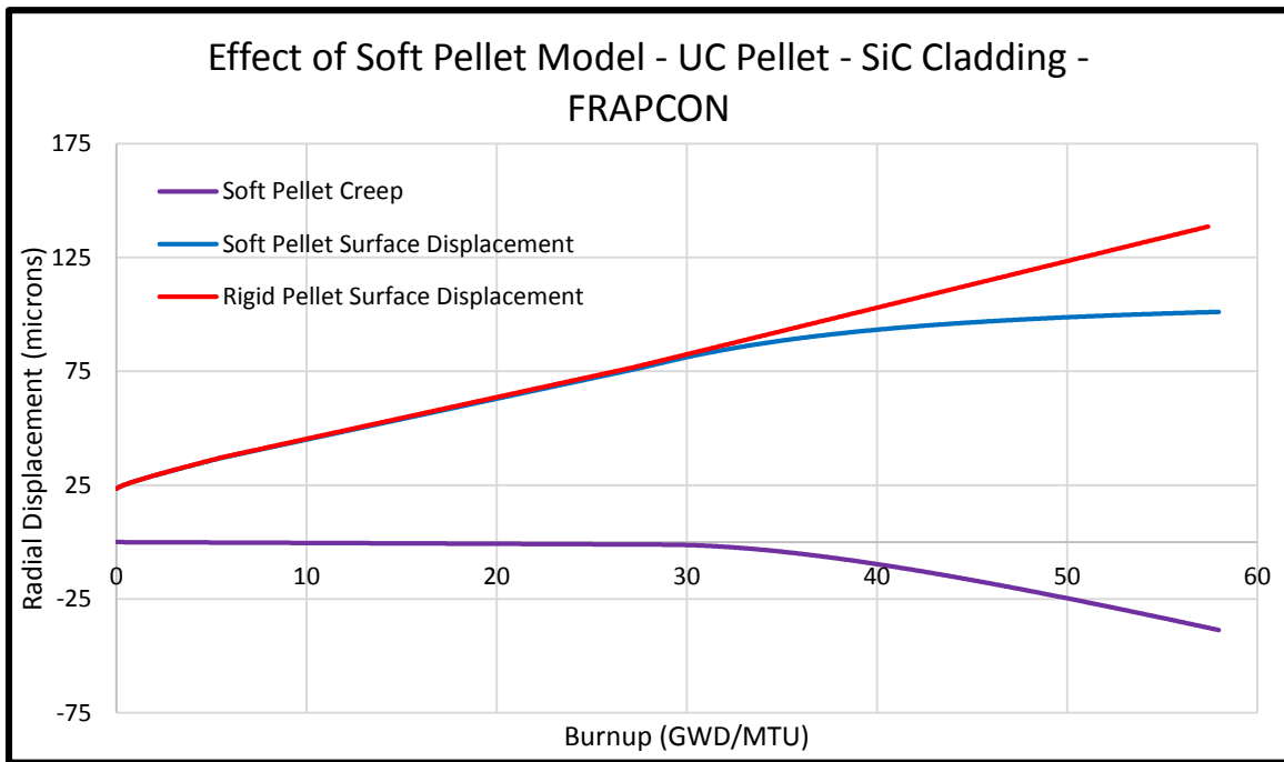
Figure 4.12: Effect of Soft Pellet Model - UC Pellet - SiC Cladding
