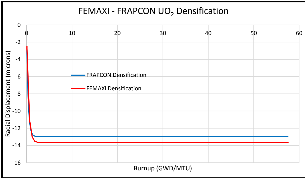
Figure 3.3: FRAPCON/FEMAXI Densification
